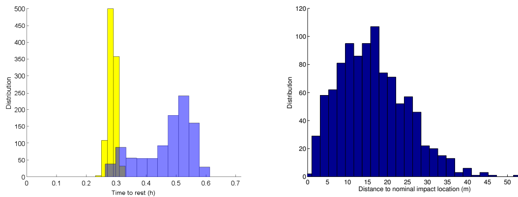
Figure 4.6: MonteCarlo simulations of a deployment to 1999 JU3 from 100m altitude, with a full stochastic model and e = 0.35 .
