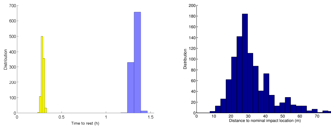
Figure 4.8: MonteCarlo simulations of a deployment to 1999 JU3 from 100m altitude, for no stochastic model and e = 0.65 .
