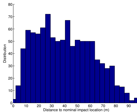
Figure 4.5: MonteCarlo simulations of a deployment to 1999 JU3 from 100m altitude, with a full stochastic model and e = 0.65 .
