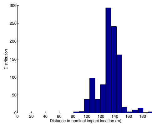
Figure 4.7: MonteCarlo simulations of a deployment to 1999 JU3 from 100m altitude, for no stochastic model and e = 0.85 .
