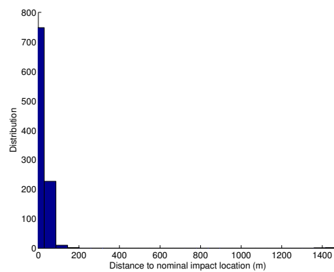
Figure 4.10: MonteCarlo simulations of a deployment to 1999 KW4 Alpha from 28m altitude.
