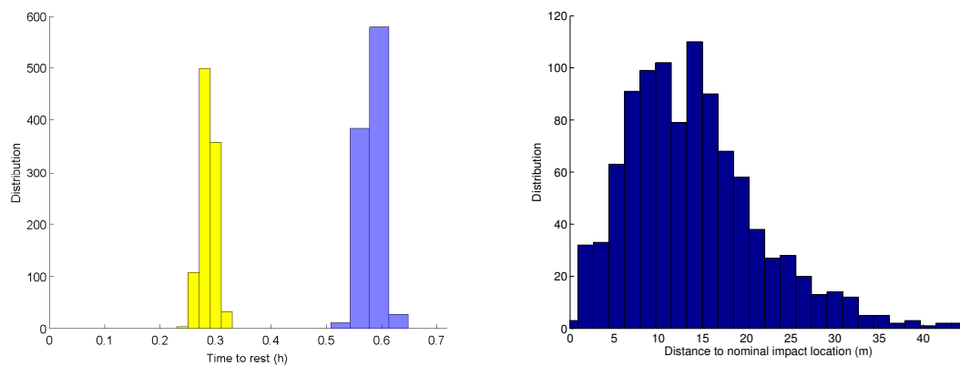
Figure 4.9: MonteCarlo simulations of a deployment to 1999 JU3 from 100m altitude, for no stochastic model and e = 0.35 .
